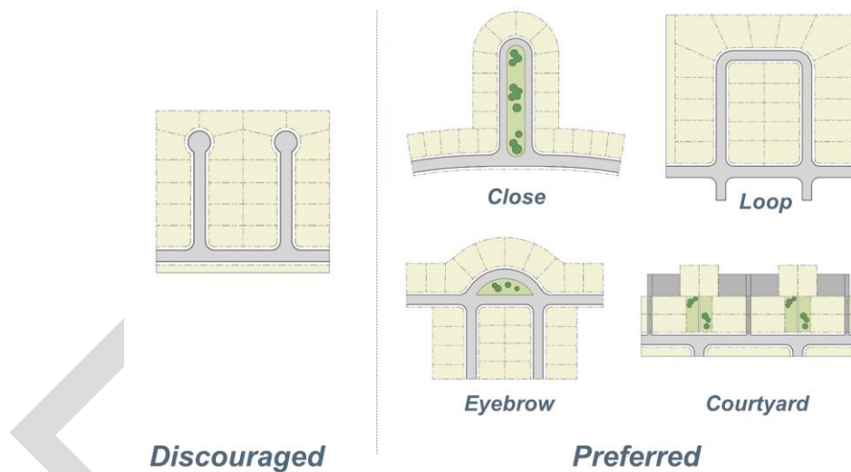
Figure 3-3 Disconnected Street Options. Where streets will not connect, blocks and lots should be laid out to limit the need for cul-de-sacs and maximize other options such as loops, closes, eyebrows and courtyard patterns. (3.01.B.2.f.)
